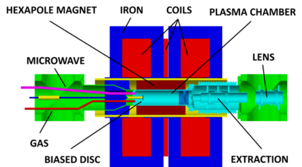
Figure 4: Schematic representation of the ECR ion source at ATOMKI
