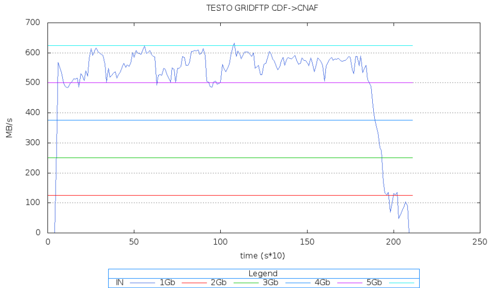
Figure 4. Results of data transfer test between FNAL and CNAF. With \sim 50 -80 parallel copy processes the available bandwidth is fully exploited.
