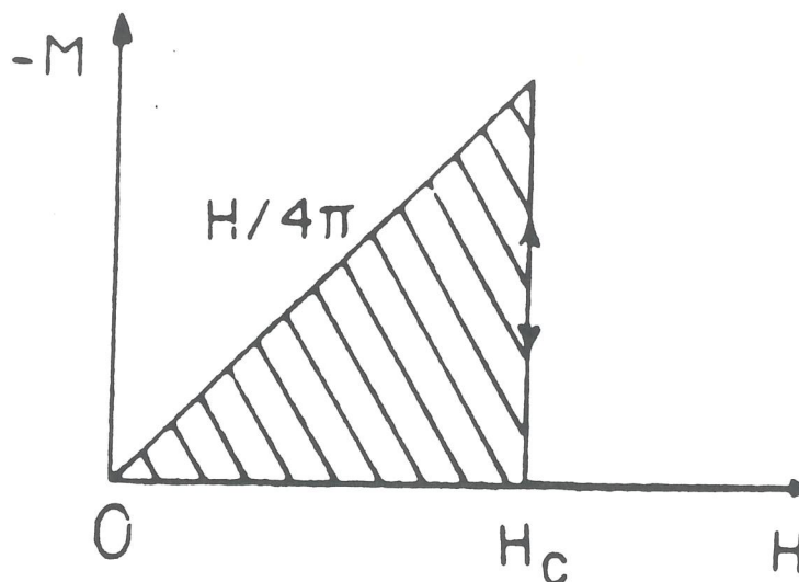
Fig, 10 The magnetization in the superconducting state is equal to -\frac{H}{4\pi} , while it is zero in the normal state.
