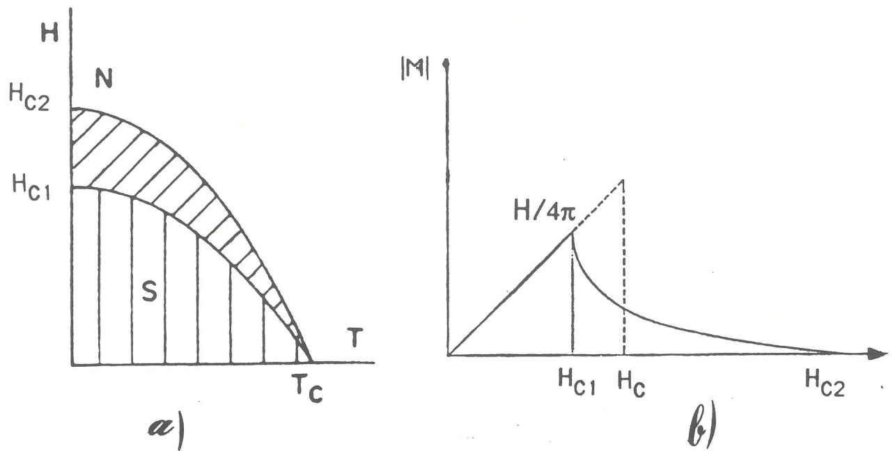
Fig 11 a) The temperature dependence of H_{C1} and H_{C2} b) The magnetization versus field for Type II superconductors clearly shows a region of incomplete Meissner Ochsenfeld effect.
