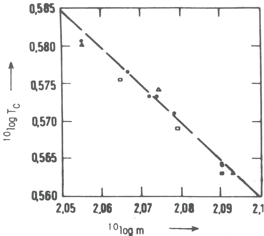
Fig. 21 The isotope effect for Sn.
