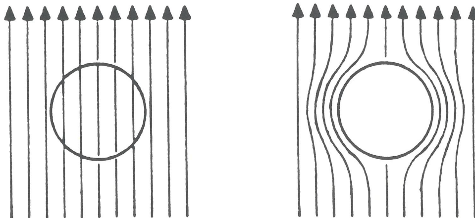
Fig. 7: The Meissner-Ochsenfeld effect: when a material undergoes the superconducting transition, the magnetic induction B is shrunk out of the sample.
