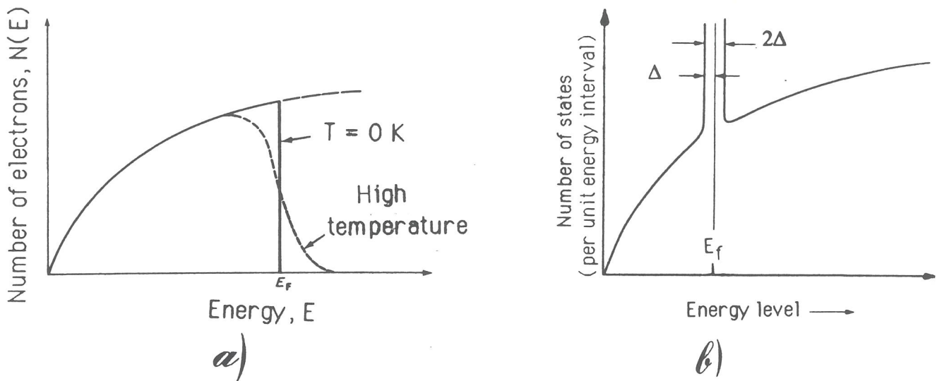
Fig. 18 The density of electron energy states versus energy a) for a normal metal b) for a superconductor.
